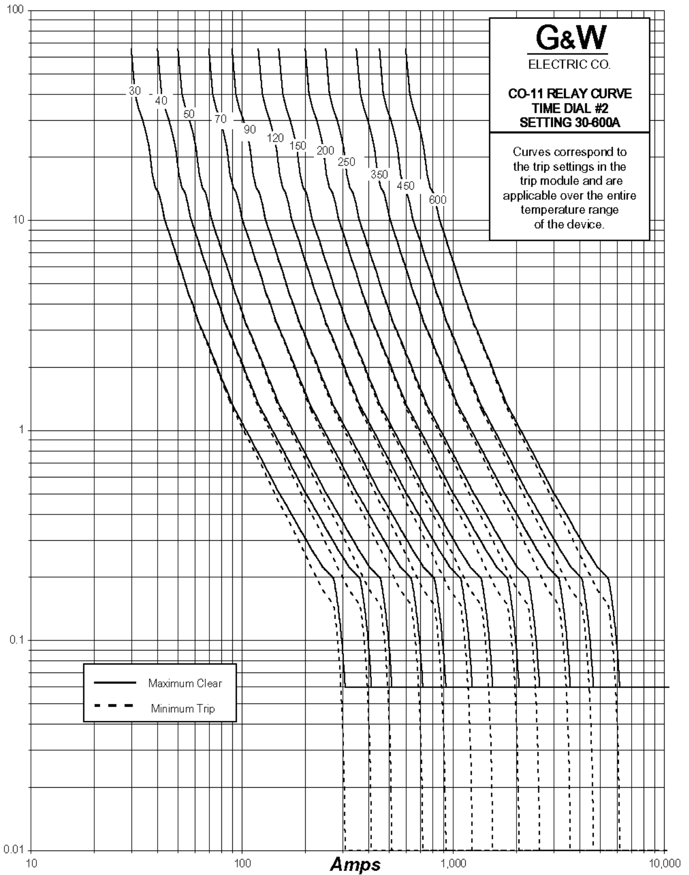
TIME – CURRENT CHARACTERISTIC CURVES FOR: Vacuum Interrupters
