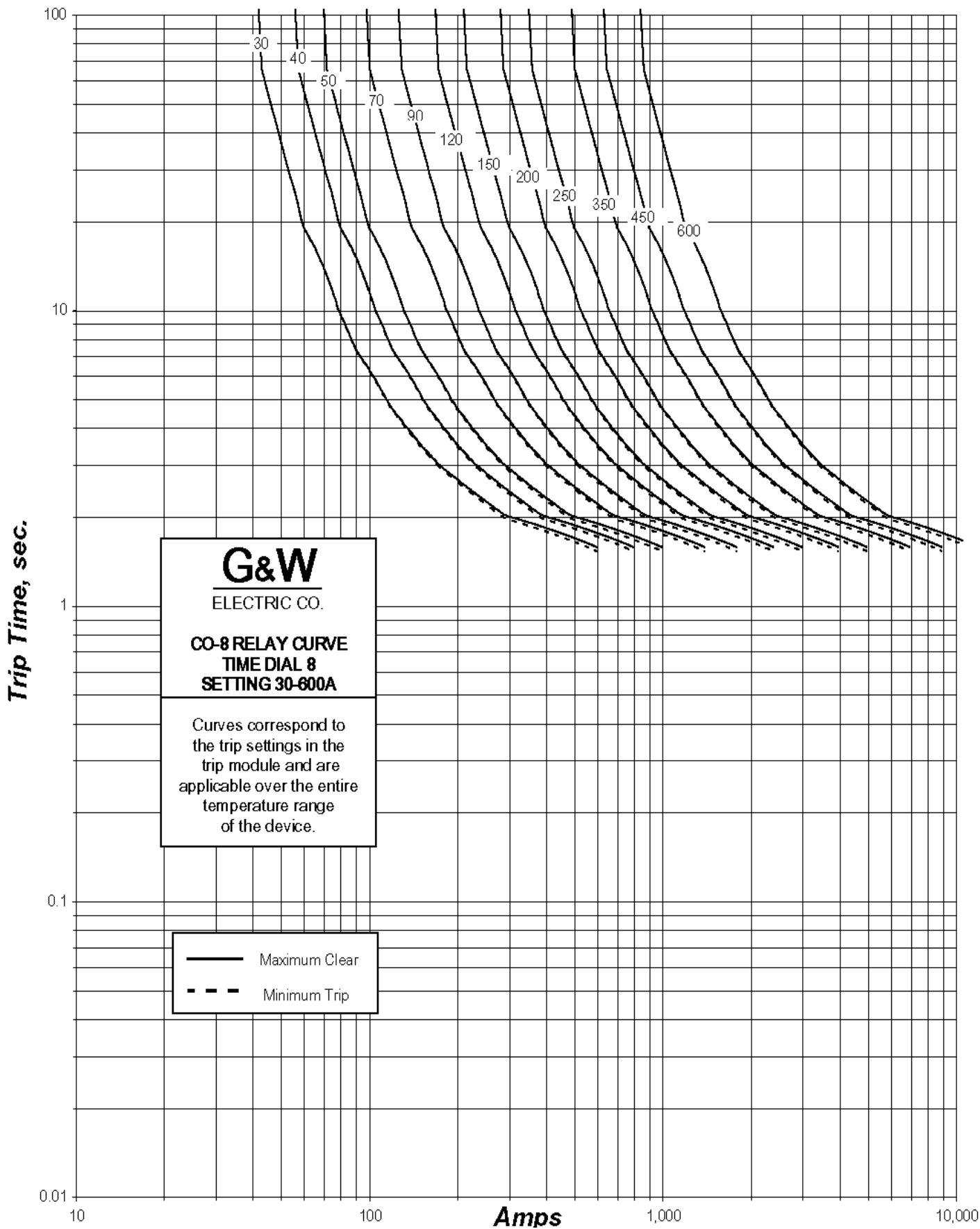
TIME – CURRENT CHARACTERISTIC CURVES FOR: Vacuum Interrupters
