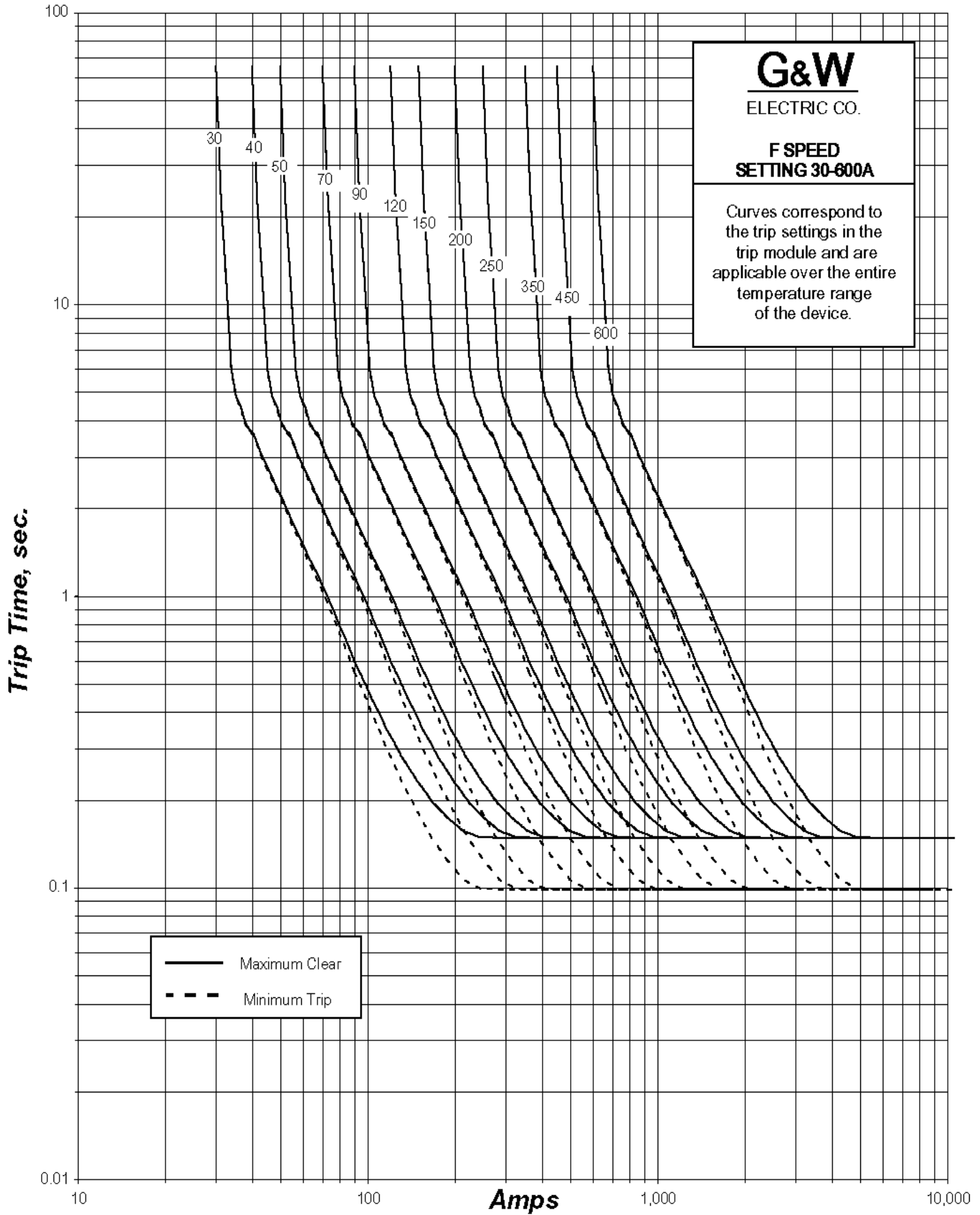
TIME – CURRENT CHARACTERISTIC CURVES FOR: Vacuum Interrupters
