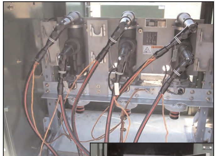
Photo above shows the recloser compartment access for cable connections.
