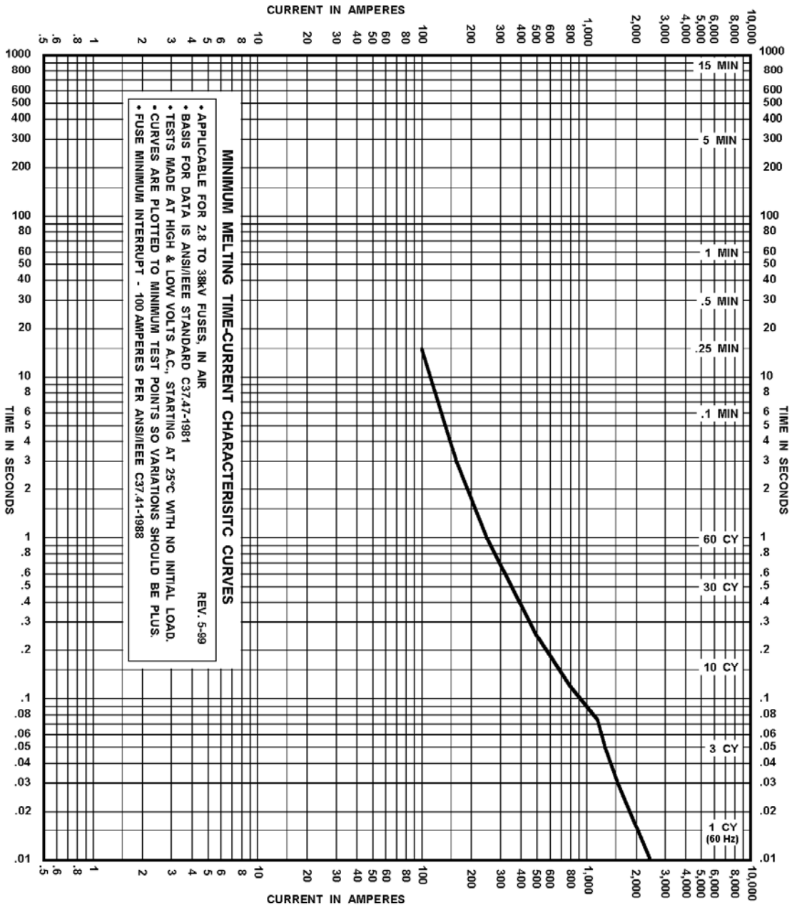
25 AMPERE, 80KA HIGH CURRENT BACK-UP LIMITER MINIMUM MELTING TIME-CURRENT CHARACTERISTIC CURVE
