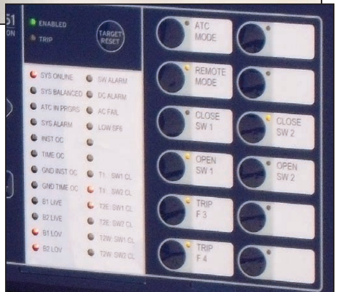
Large, clearly labeled pushbuttons provide an easy way for facilities personnel to operate individual switches safely and with confidence.
