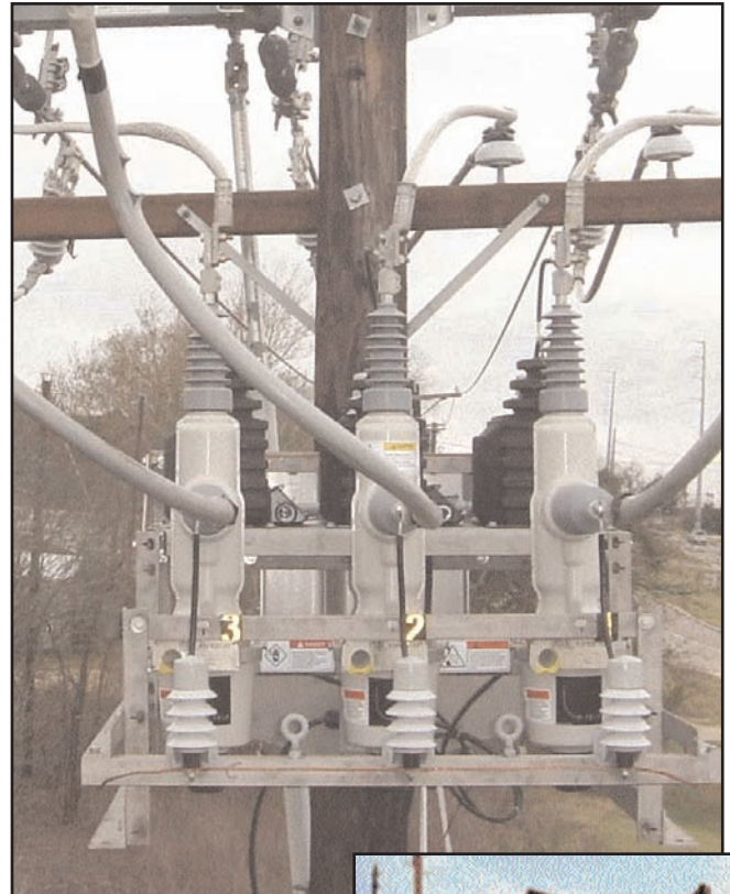
Figure 1 above: Pole mounted, 15kV Viper-ST recloser.
